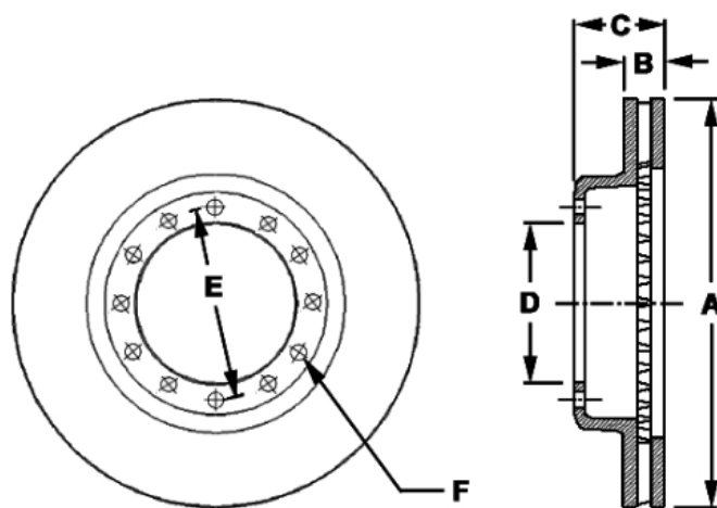
Rotor Configuration
