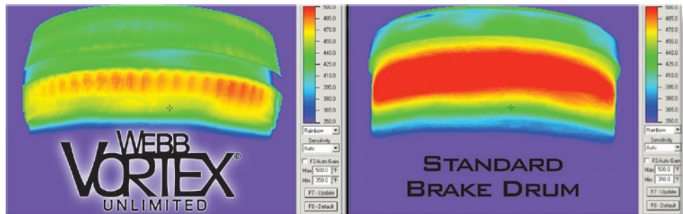
These photos taken from an infra-red camera mounted on the Webb dyno show a Webb Vortex® Unlimited drum next to a standard drum at precisely the same moment during braking. Compare the heat (red color) and you can actually see that Webb Vortex® Unlimited brake drums run significantly cooler.
