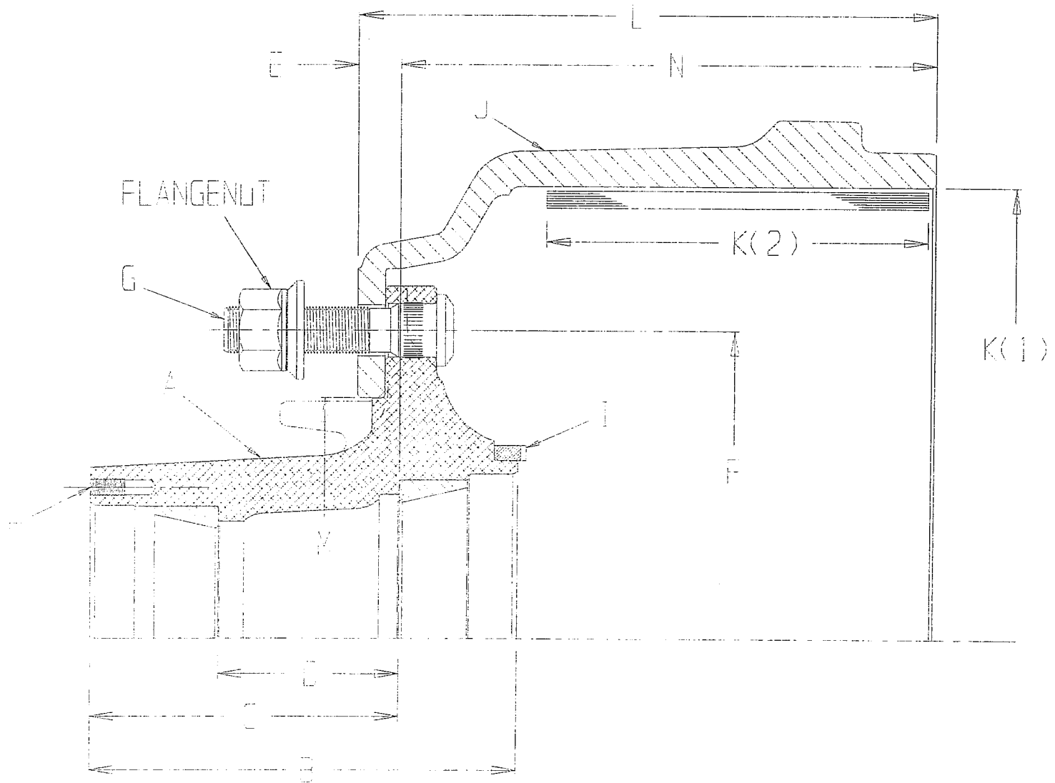
Assembly Drawing
